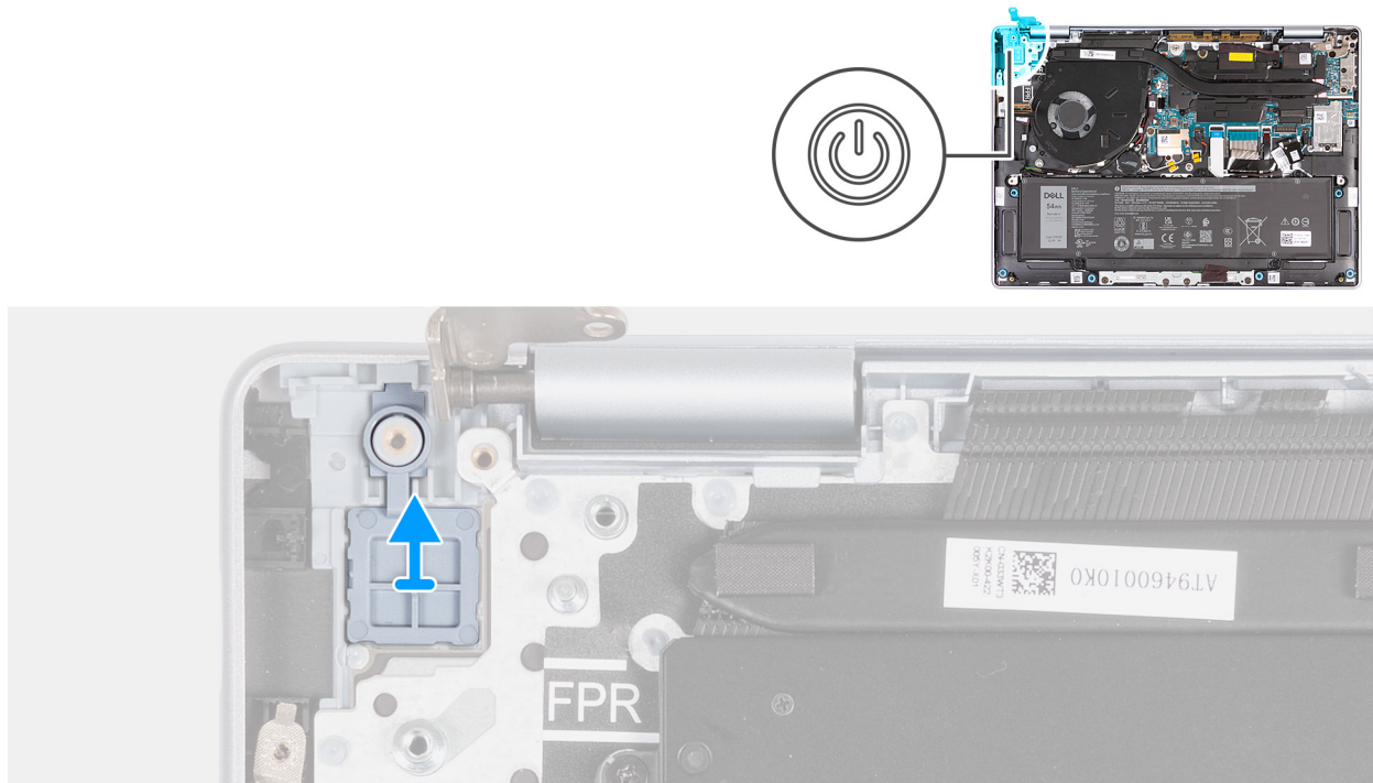
Figure 46. Removing the power button
