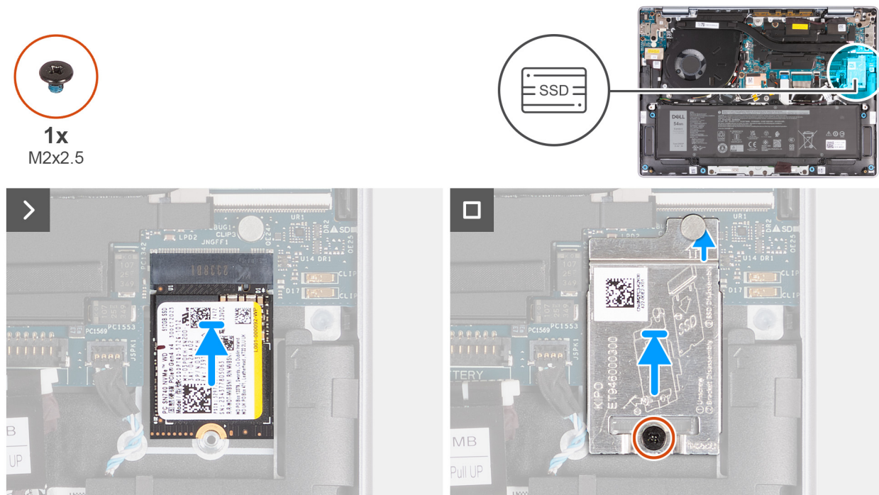
Figure 20. Installing the solid state drive
