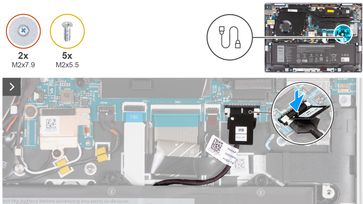
Figure 14. Connecting the battery cable
