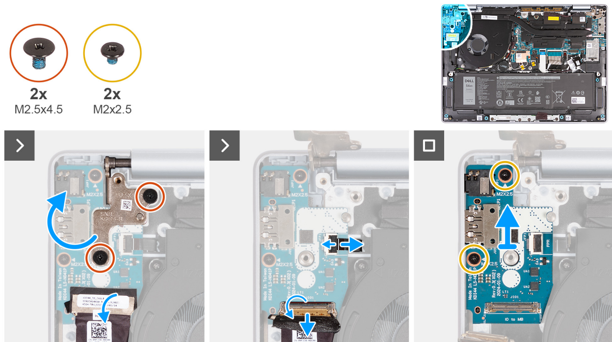
Figure 40. Removing the I/O board
