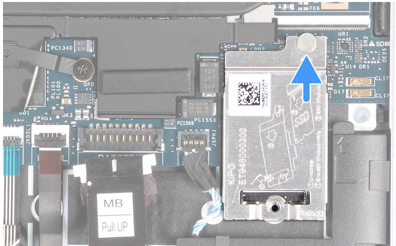
Figure 22. Installing solid state drive thermal shield
