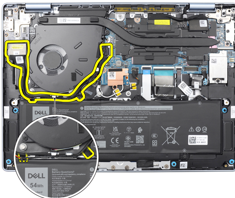
Figure 43. I/O-board cable routing
