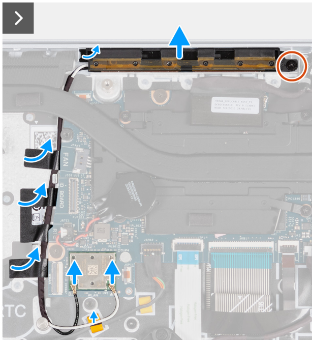
Figure 52. Removing the antennas
