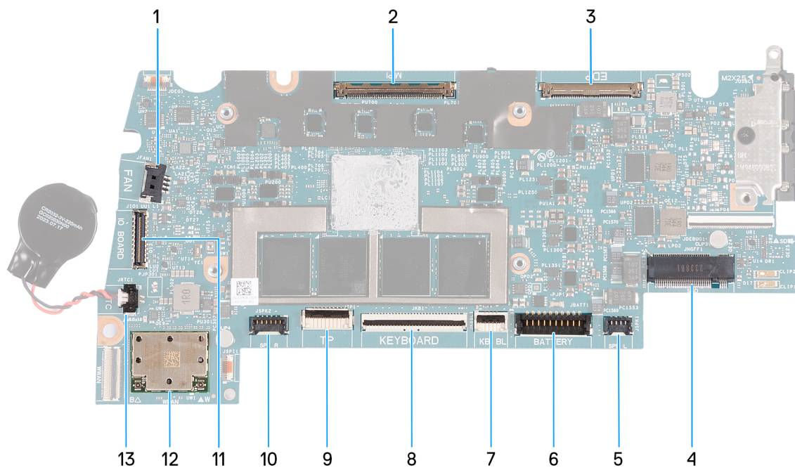
Figure 58. System board connectors
