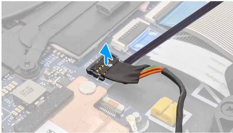
Figure 24. Disconnecting speaker cable
