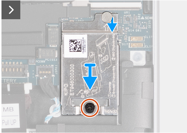
Figure 19. Removing the solid state drive
