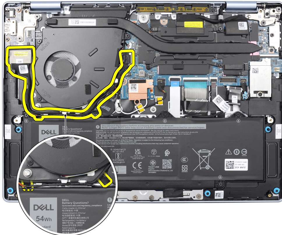
Figure 45. I/O-board cable routing
