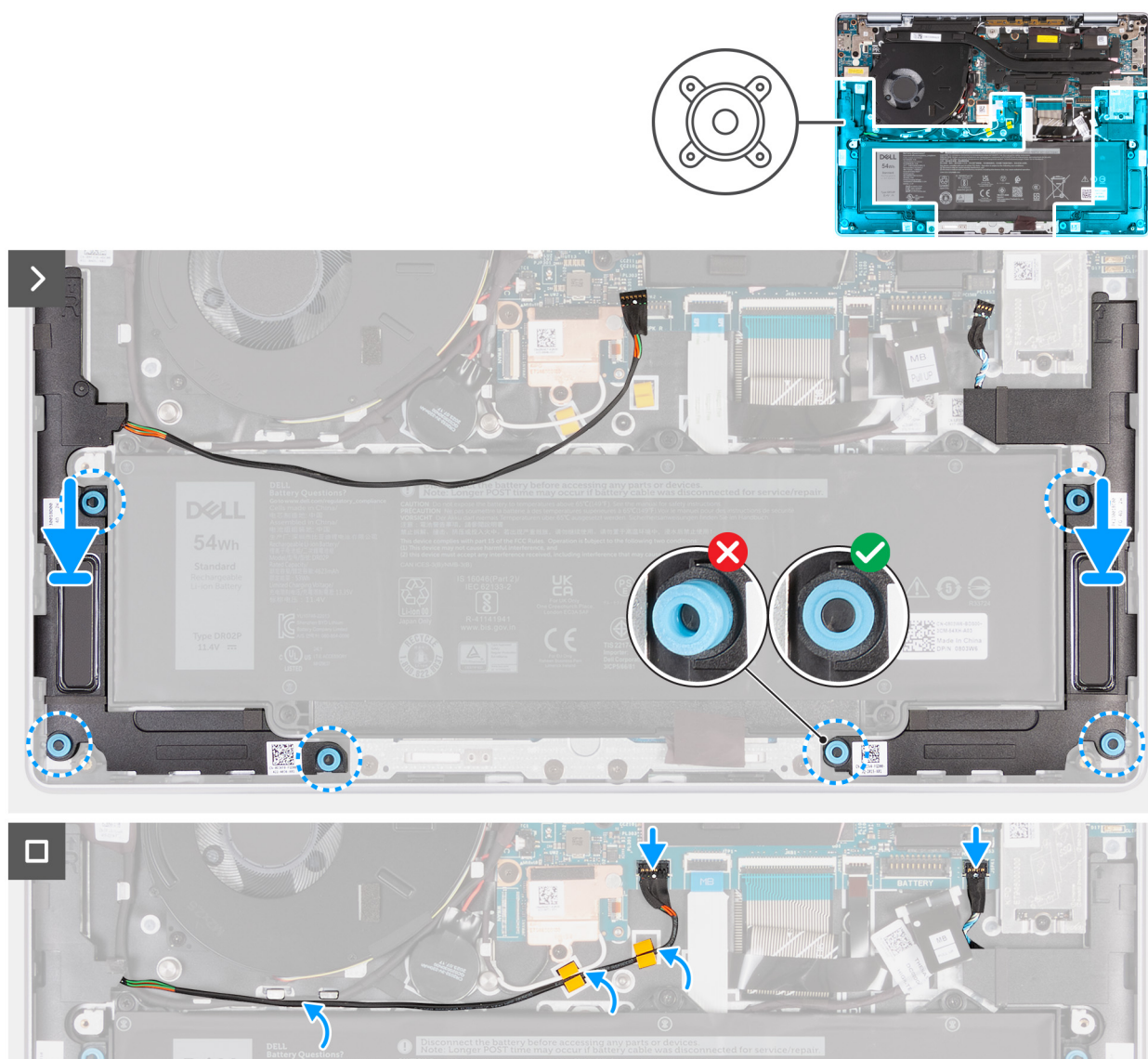
Figure 25. Installing the speakers
