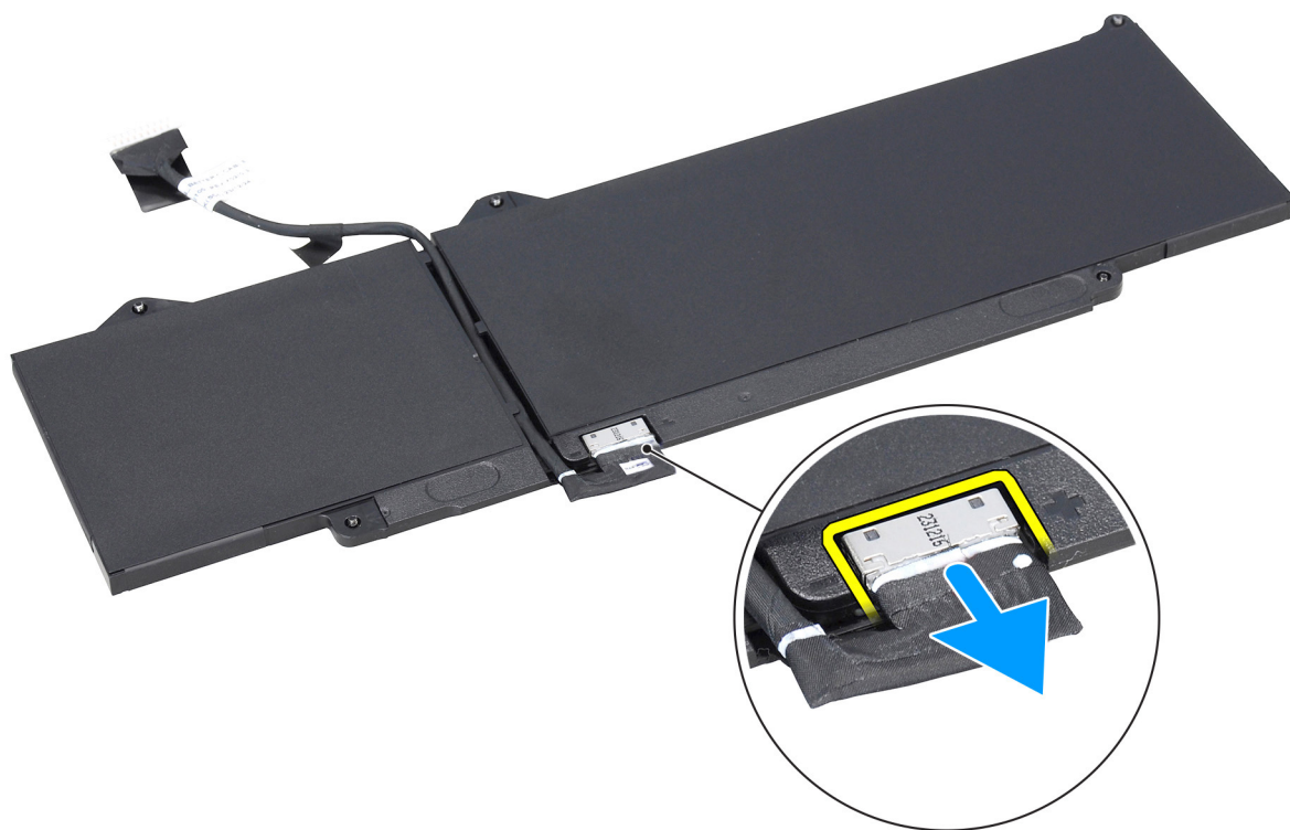
Figure 29. Disconnecting the battery cable
