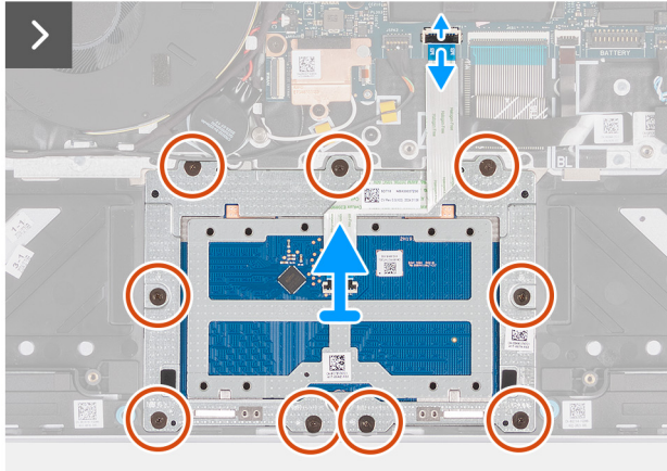
Figure 38. Removing the touchpad
