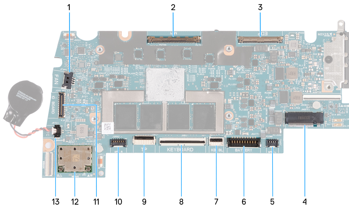
Figure 61. System board connectors
