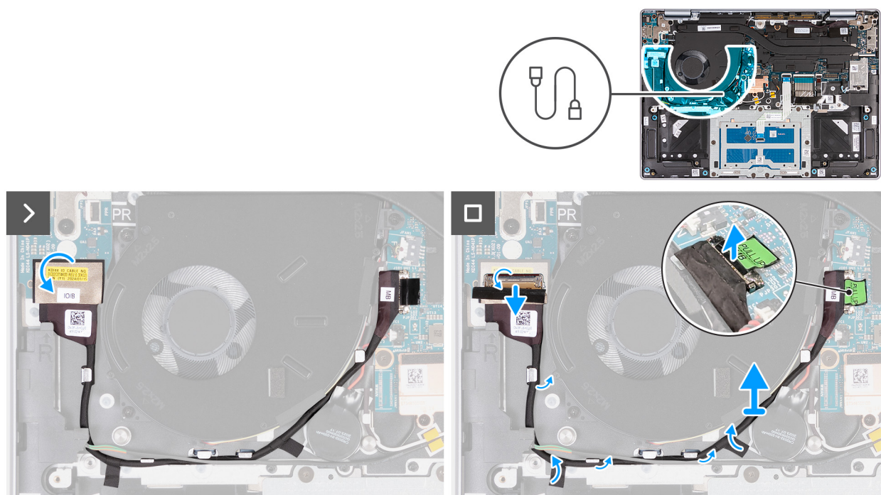
Figure 42. Removing the I/O-board cable
