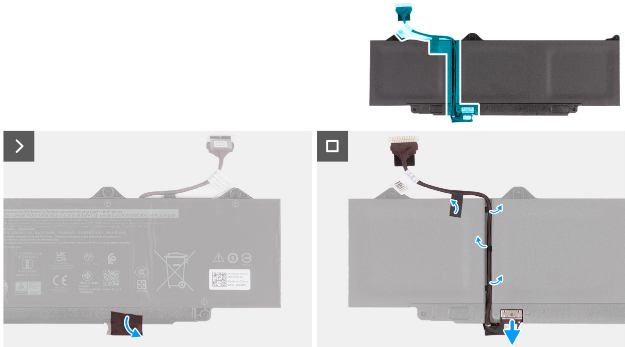
Figure 28. Disconnecting the battery cable
