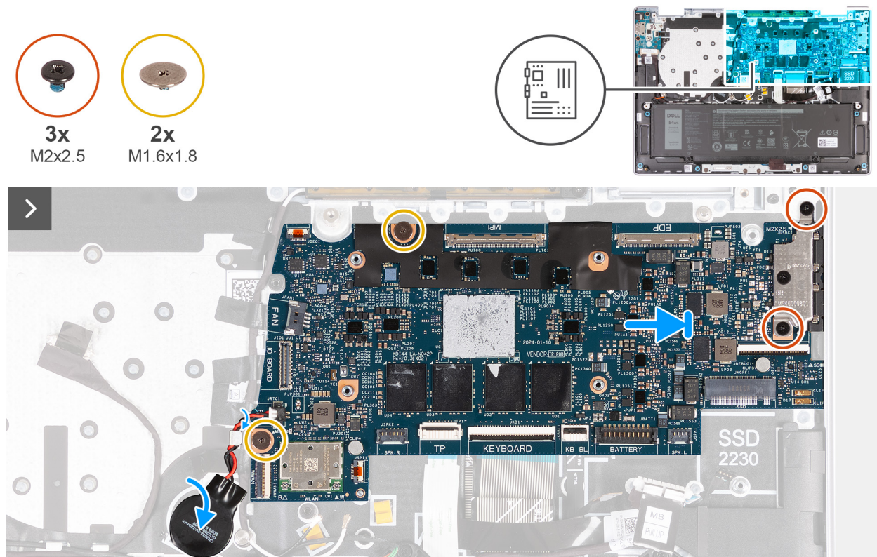
Figure 62. Installing the system board
