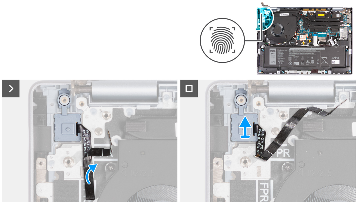
Figure 49. Removing the power button with optional fingerprint reader
