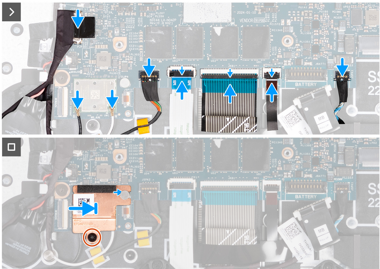
Figure 63. Connecting the cables
