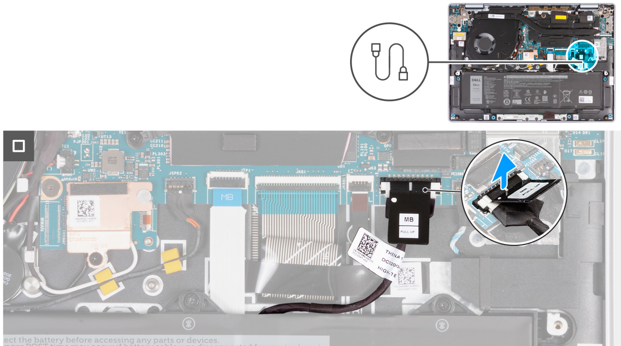
Figure 13. Disconnecting the battery cable
