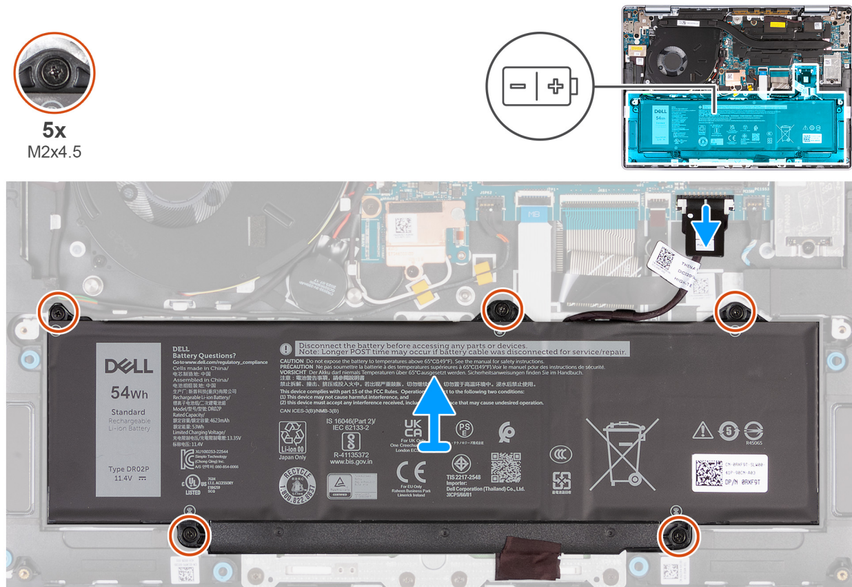
Figure 26. Removing the battery
