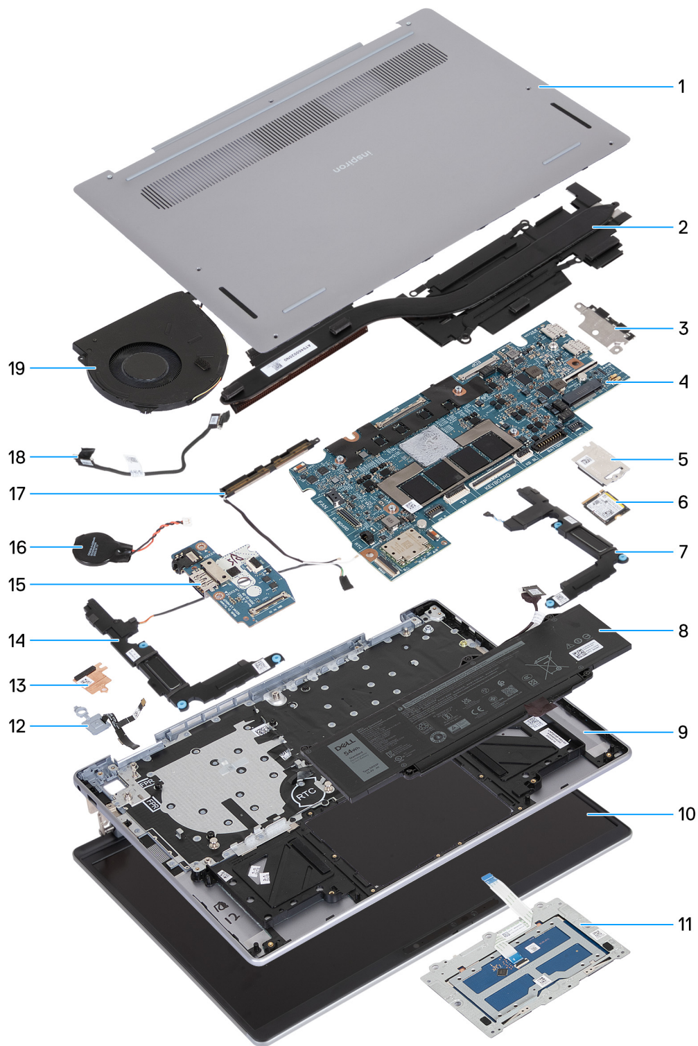
Figure 10. Major components
