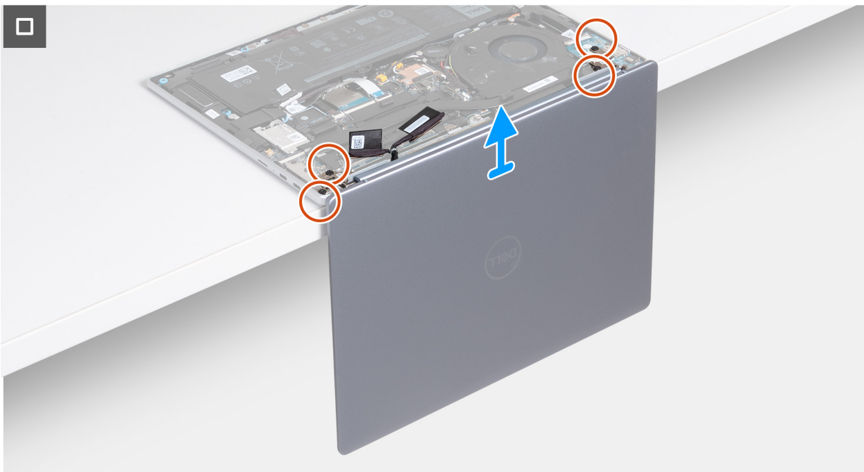
Figure 33. Removing the display assembly
