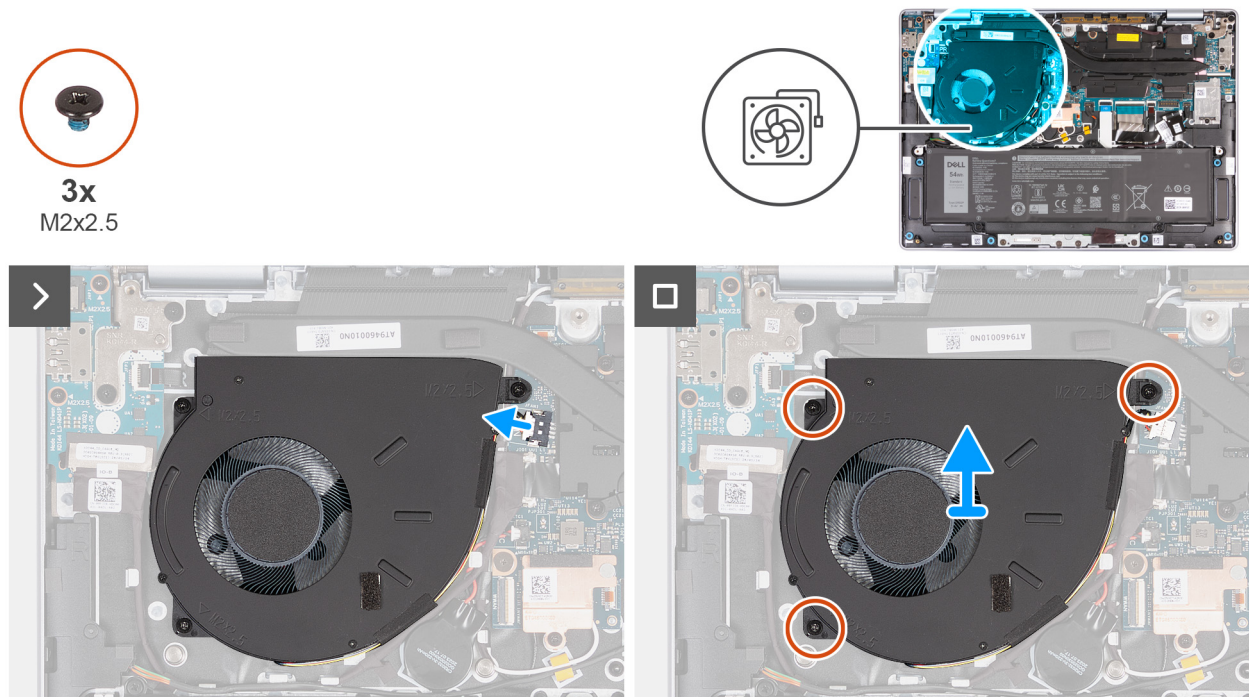
Figure 17. Removing the fan
