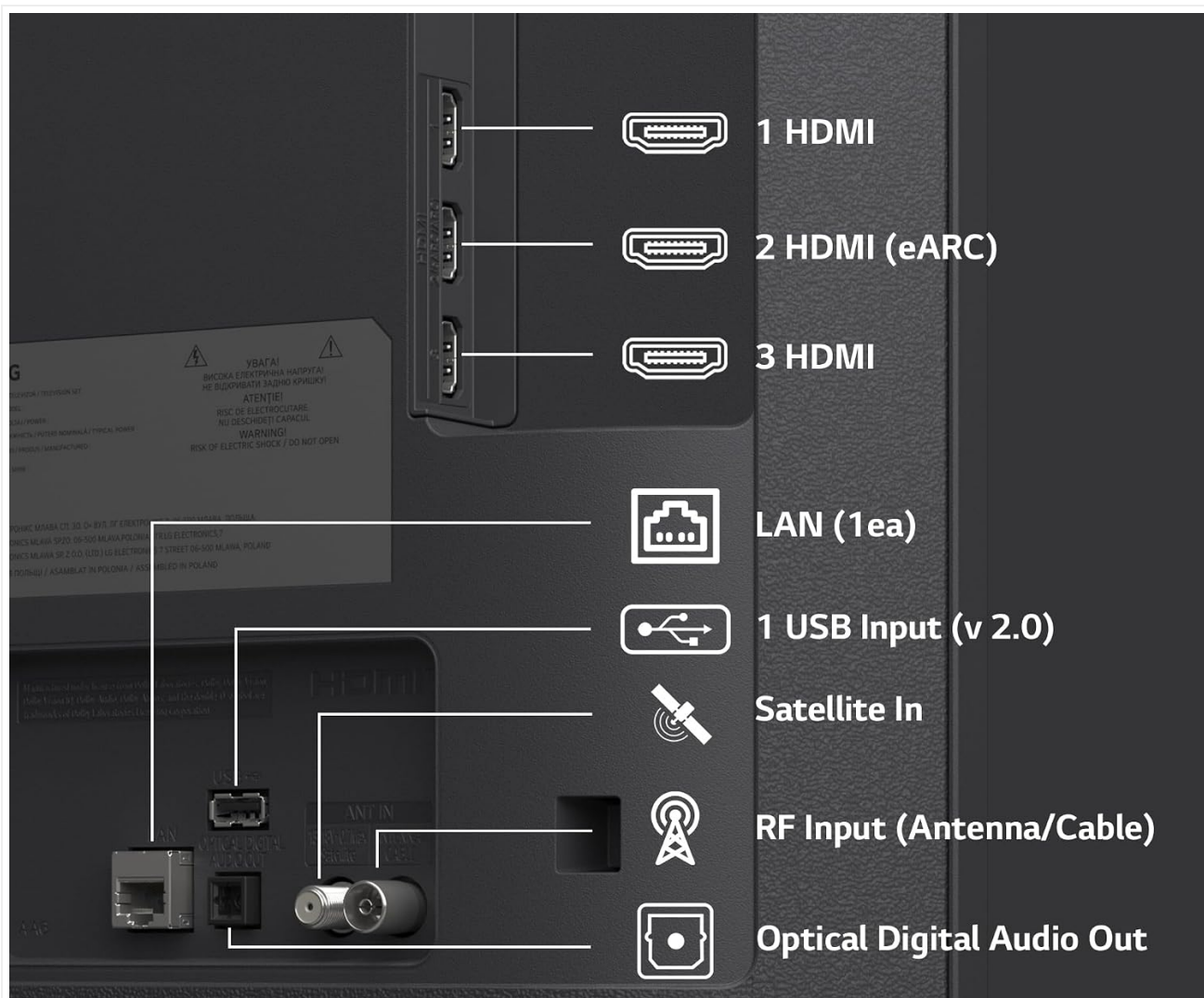
Image 2.3: Rear view of the LG TV showing connectivity ports: 3 HDMI ports (one with eARC), 1 LAN (Ethernet), 1 USB Input (v 2.0), Satellite In, RF Input (Antenna/Cable), and Optical Digital Audio Out.
