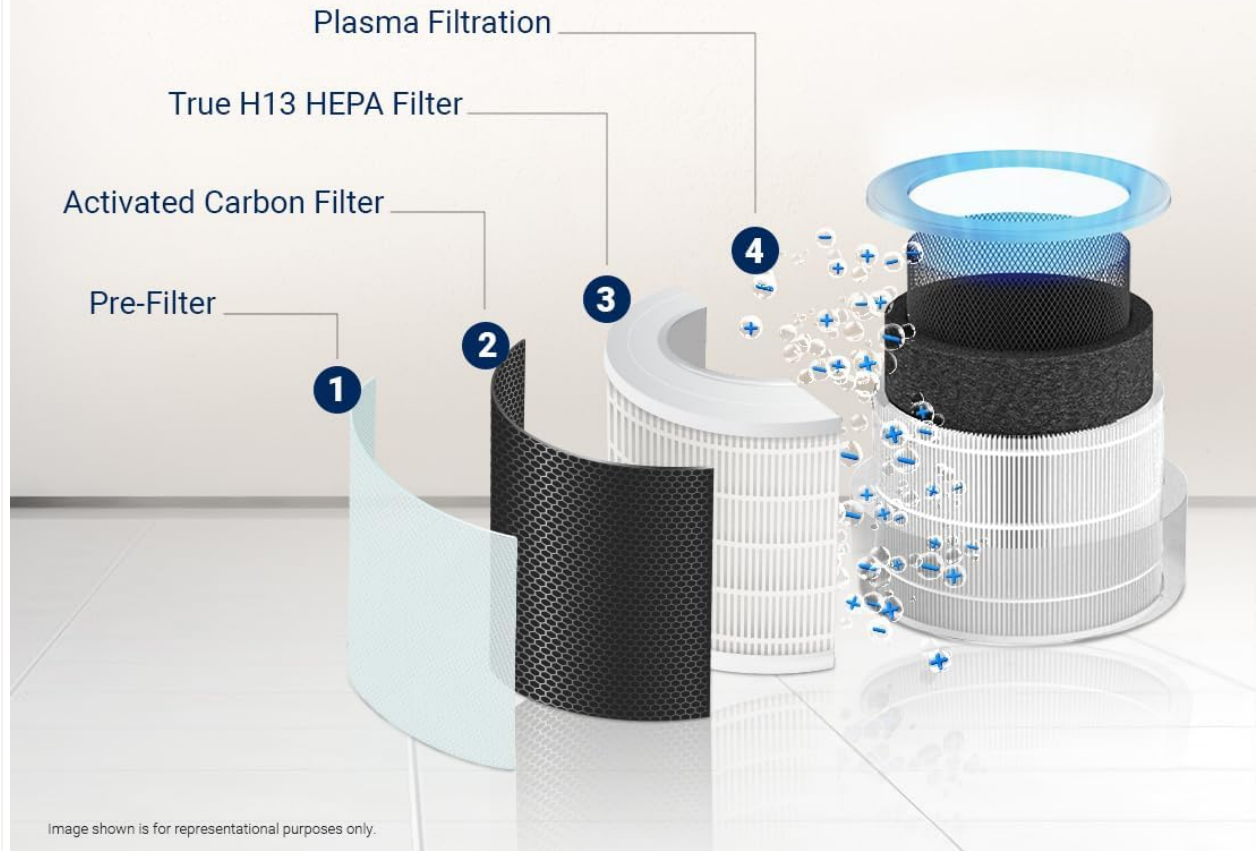
Figure 3.3: Exploded view of the 4-stage filtration system.
